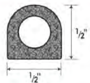
D-Profile S0202 Series
