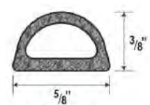
D-Profile S0109 Series
