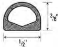
D-Profile S0108 Series
