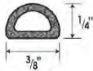
D-Profile S1153 Series
