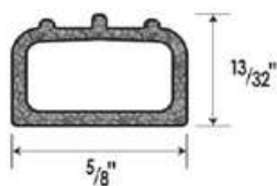
Ribbed Profile S1705 Series
