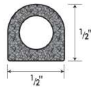
D-Profile S0202 Series
