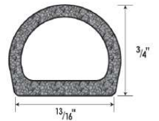
D-Profile S1750 Series
